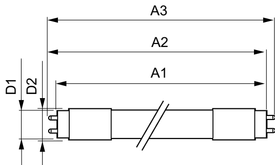
LEDtube 1500mm UO 25W 840 T8 ROT
